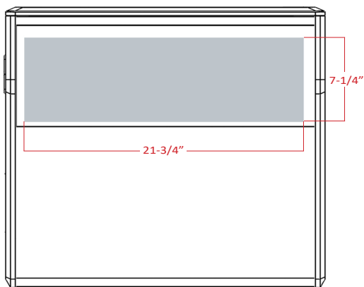
Flat Surface Configuration 5" Depth
